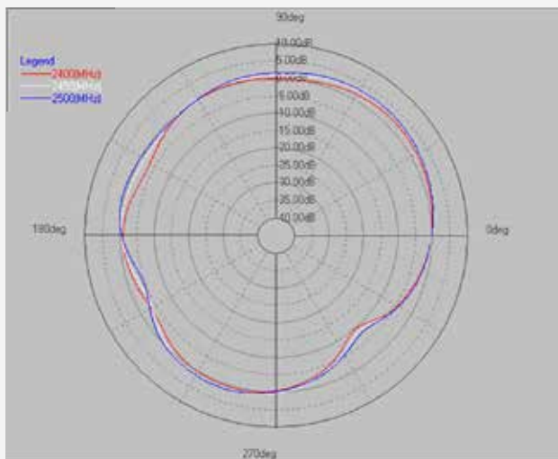
2.4G (PHI=0)
