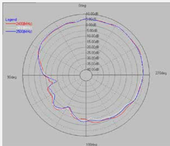
2.4G (PHI=90)
